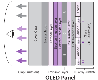
OLED Panel
